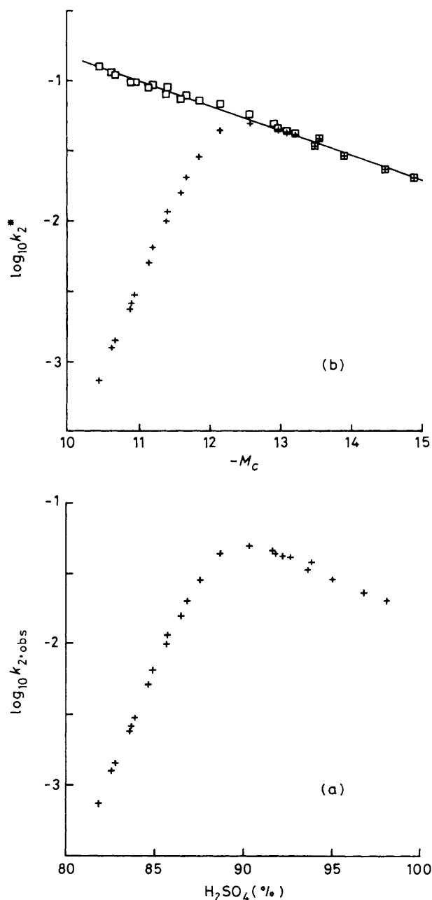
Figure 1. Rate profiles for nitration in 80–98 wt% \text{H}_2\text{SO}_4 of nitrobenzene at 25 °C using [\text{A}_R]_{\text{st}} = 10^{-4} \text{ mol dm}^{-3} and [\text{HNO}_3]_{\text{st}} = 10^{-1} - 10^{-2} \text{ mol dm}^{-3} . (a) Values of \log k_{2,\text{obs}} vs. wt% \text{H}_2\text{SO}_4 ( k_{2,\text{obs}} in \text{dm}^3 \text{ mol}^{-1} \text{ s}^{-1} ). (b) (+) Values of \log k_{2,\text{obs}} vs. M_c ; (□) values of \log k_2^* vs. M_c (see text).
